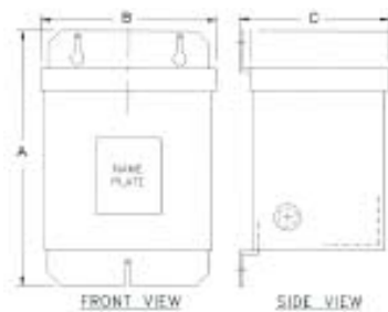
Enclosure for .10-3 KVA
