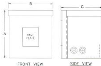
Enclosure for 5 KVA
