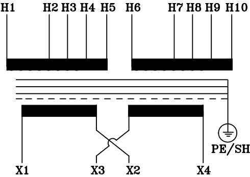
TYPICAL WIRING DIAGRAM
