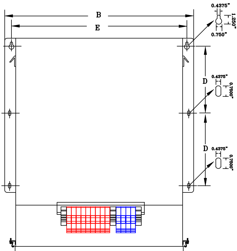
FRONT VIEW
