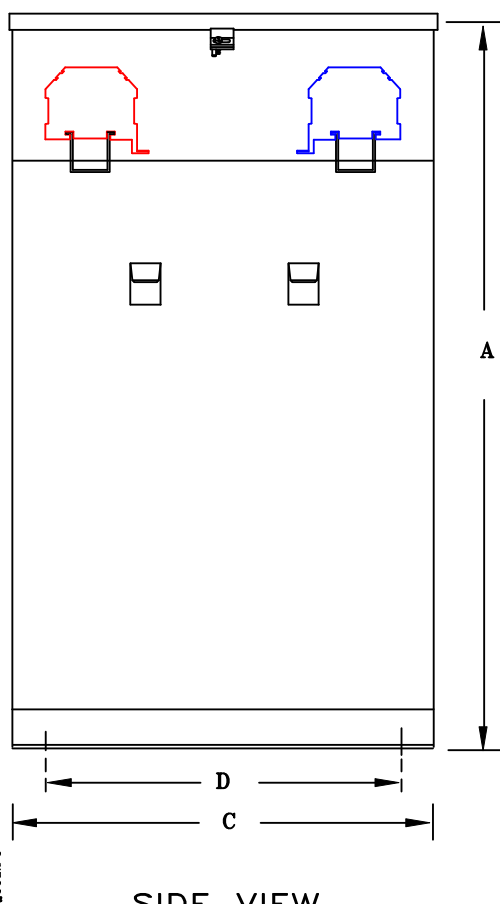
SIDE VIEW
