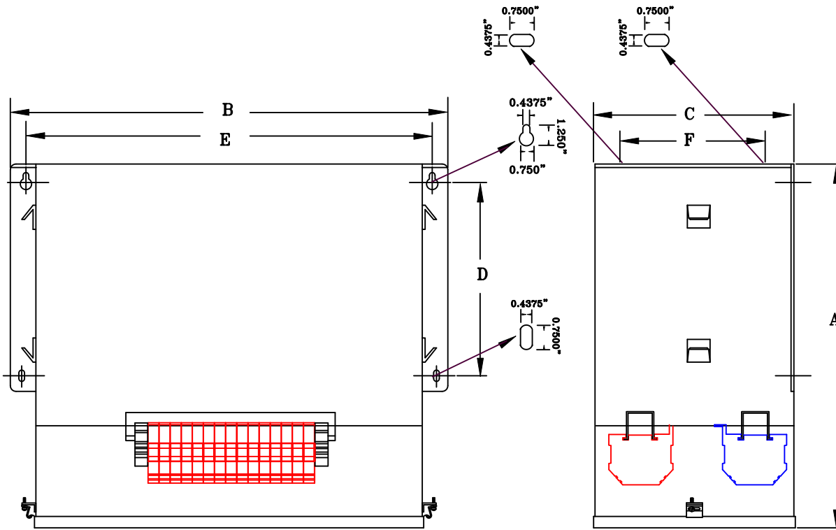
FRONT VIEW
